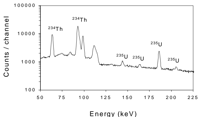
Figure 1. Gamma spectrum of the DU penetrator
