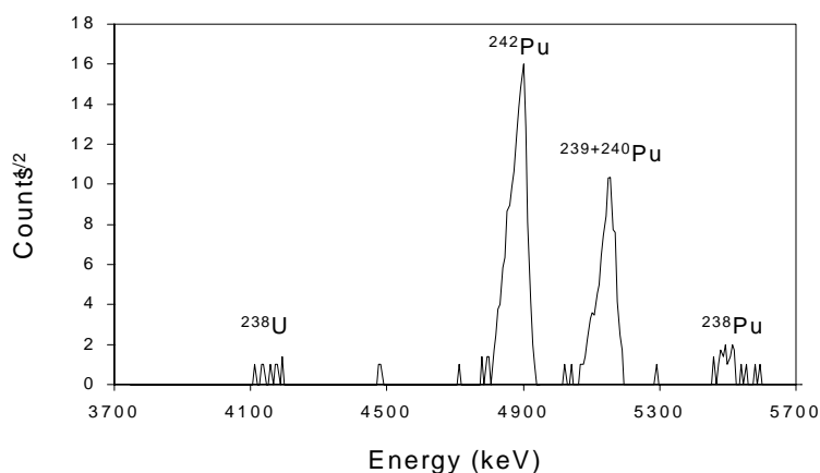
Figure 3. Pulse height spectrum of plutonium from the DU penetrator following TIOA solvent extraction
