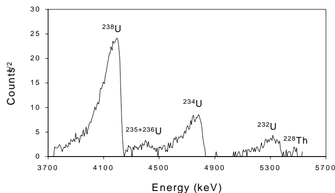
Figure 2. Pulse height spectrum of uranium from the DU penetrator
